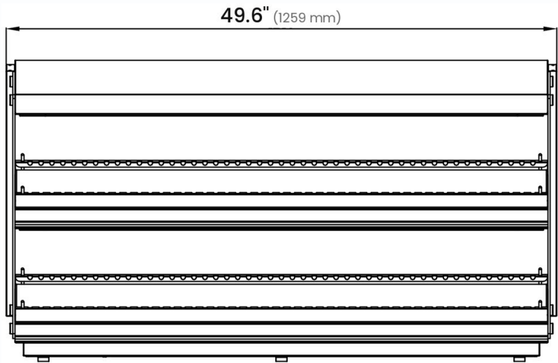
ITEM 47513 • 50" WARMER
